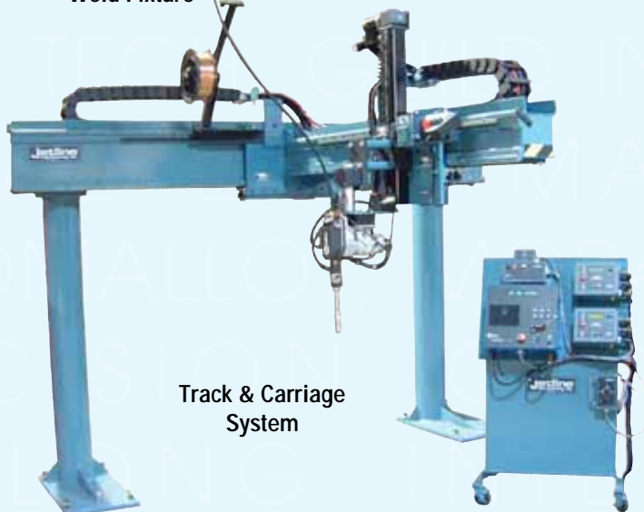
Circumferential Weld Fixture
