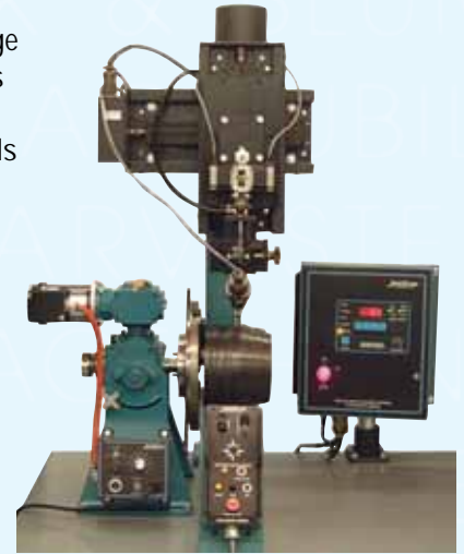
Cyclomatic Tactile Seam Tracker with ZB-300 Benchmaster Positioner
